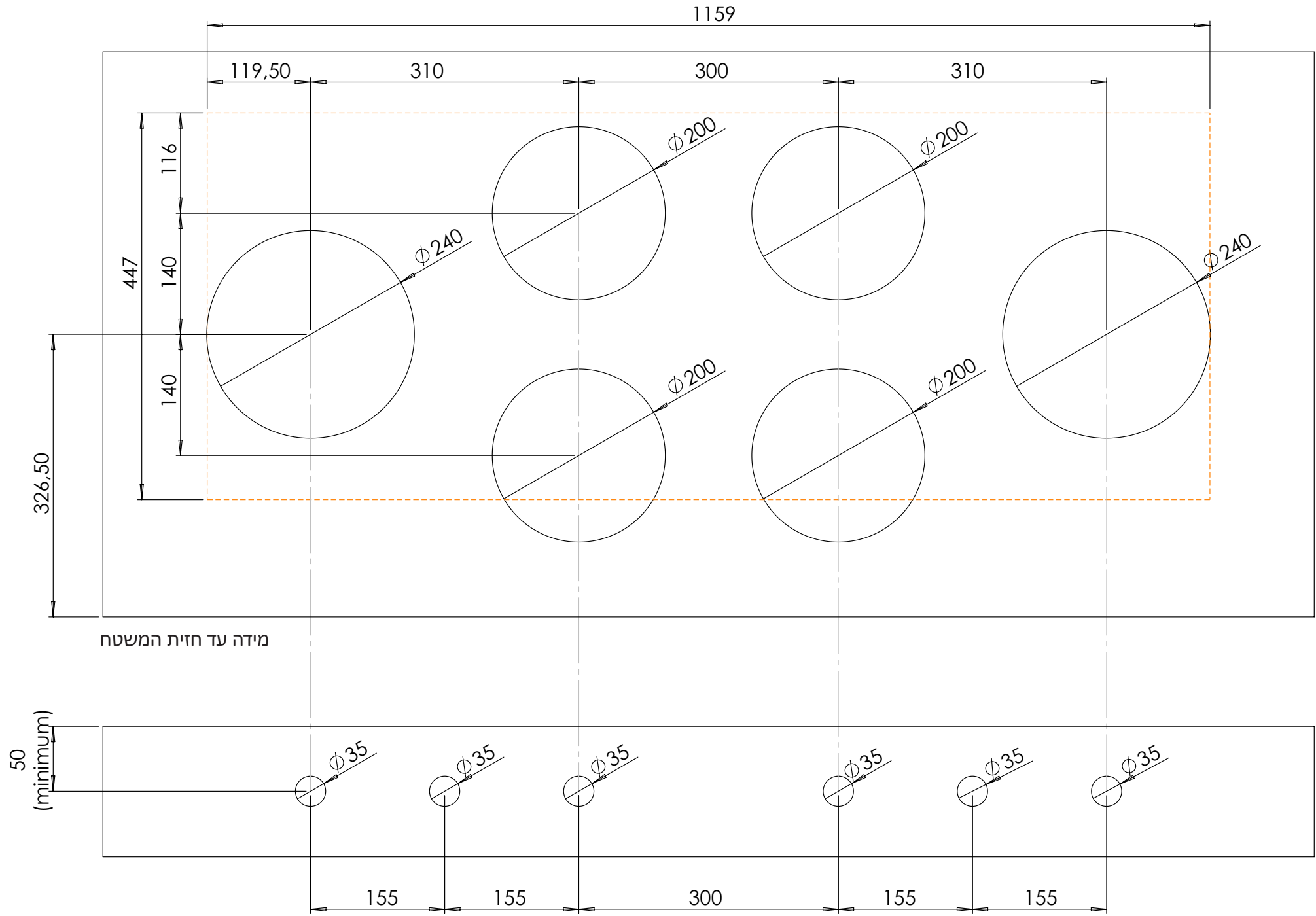
Hole pattern DXF file
